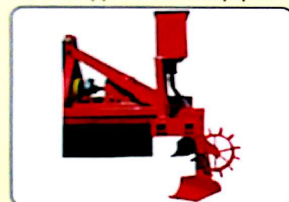
Ridges Cutting Disc (Optional)
