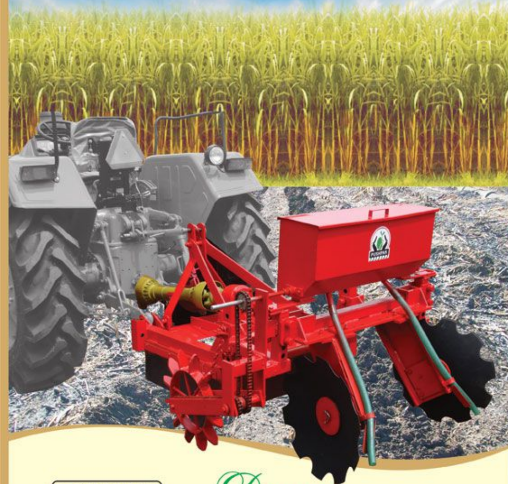
Fertilizer Application Unit (Optional)
